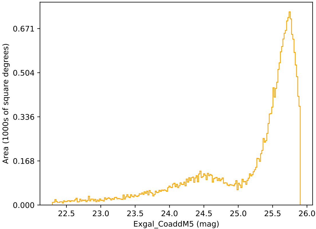
ddf_acor_sf15_lsf40_lsr20_v3.4_10yrs Yr 1 r band: Exgal_CoaddM5
