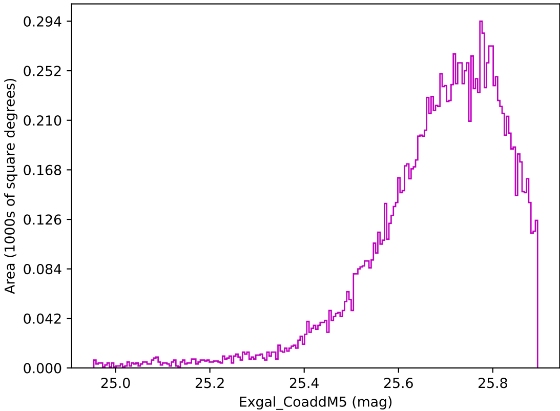
ddf_acor_sf15_lsf40_lsr20_v3.4_10yrs WFD z band: Exgal_CoaddM5
