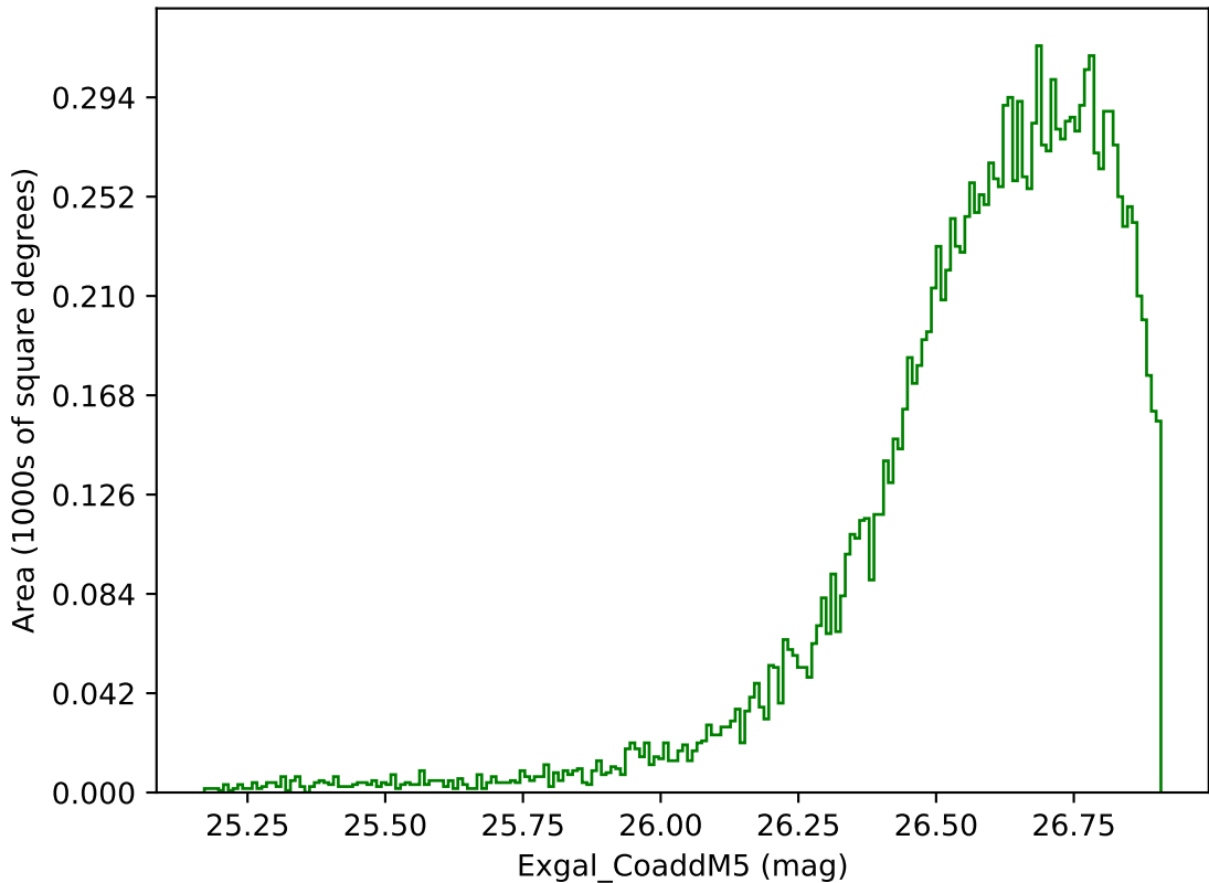
ddf_acor_sf15_lsf40_lsr20_v3.4_10yrs WFD g band: Exgal_CoaddM5
