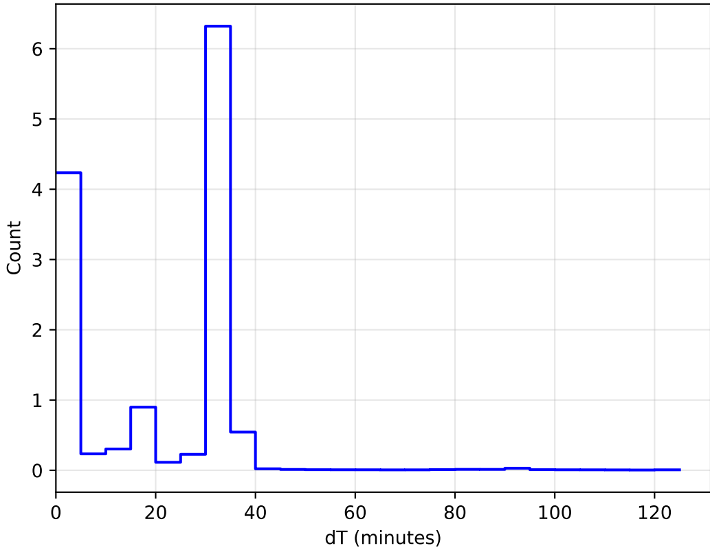
ddf_acor_sf15_lsf40_lsr20_v3.4_10yrs All sky: DeltaT Histogram
