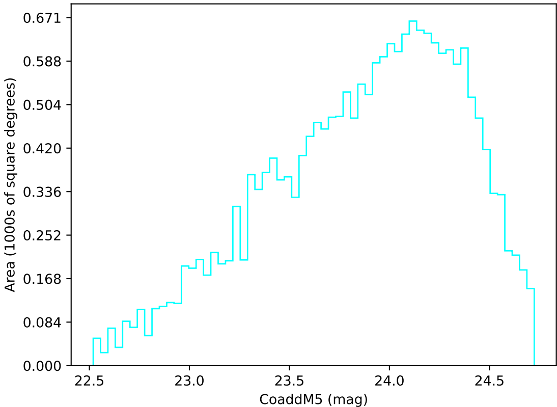
ddf_acor_sf15_lsf40_lsr20_v3.4_10yrs Yr 3-4 u band: CoaddM5
