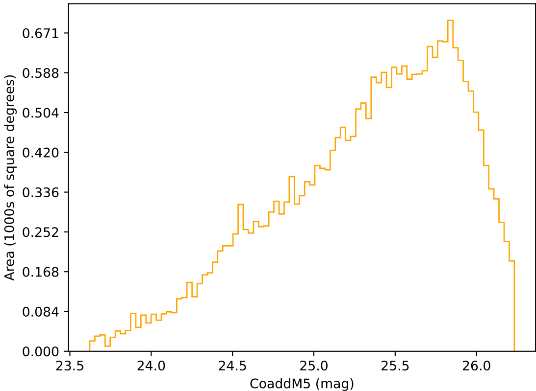
ddf_acor_sf15_lsf40_lsr20_v3.4_10yrs Yr 3-4 r band: CoaddM5
