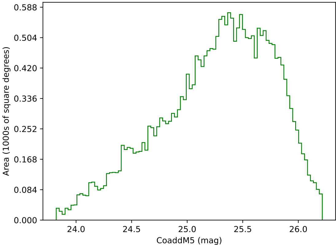
ddf_acor_sf15_lsf40_lsr20_v3.4_10yrs Yr 3-4 g band: CoaddM5
