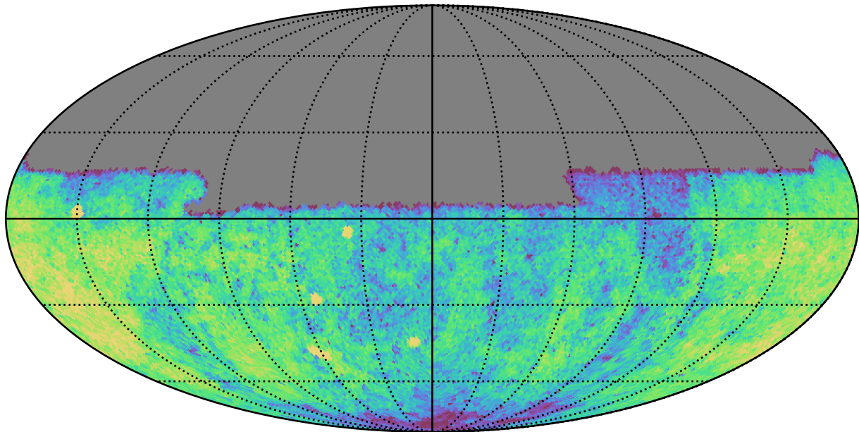
ddf_acor_sf15_lsf40_lsr20_v3.4_10yrs Yr 1 u band: CoaddM5
