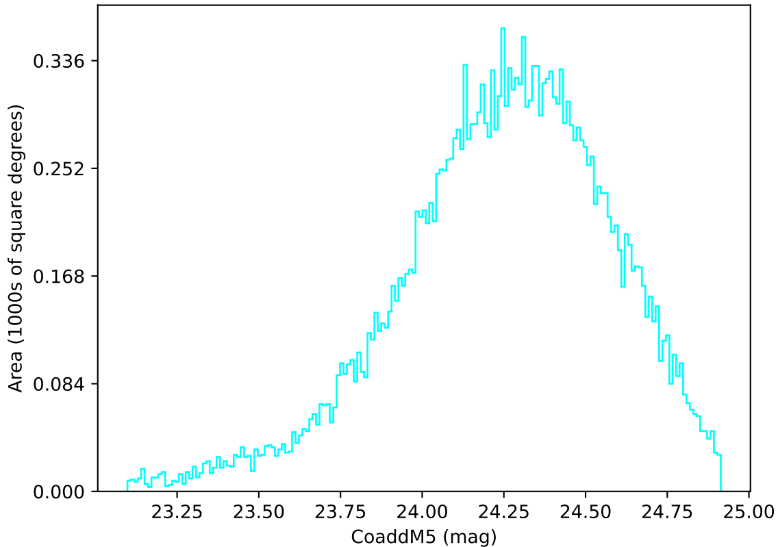
ddf_acor_sf15_lsf40_lsr20_v3.4_10yrs Yr 1 u band: CoaddM5
