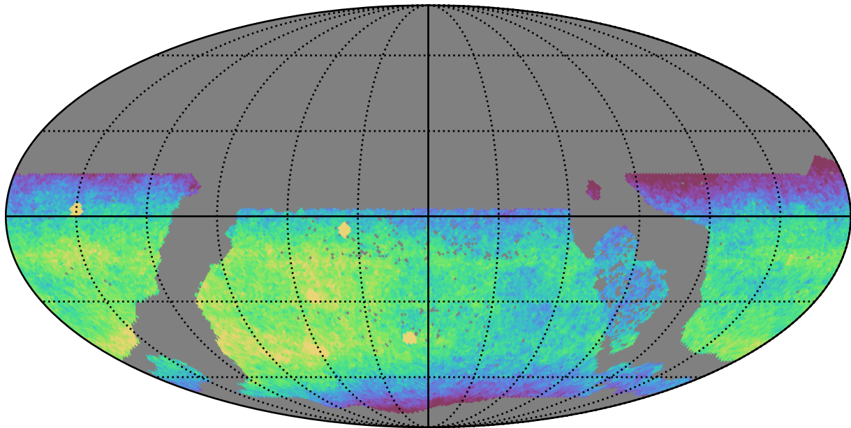
ddf_acor_sf15_lsf40_lsr20_v3.4_10yrs WFD z band: CoaddM5
