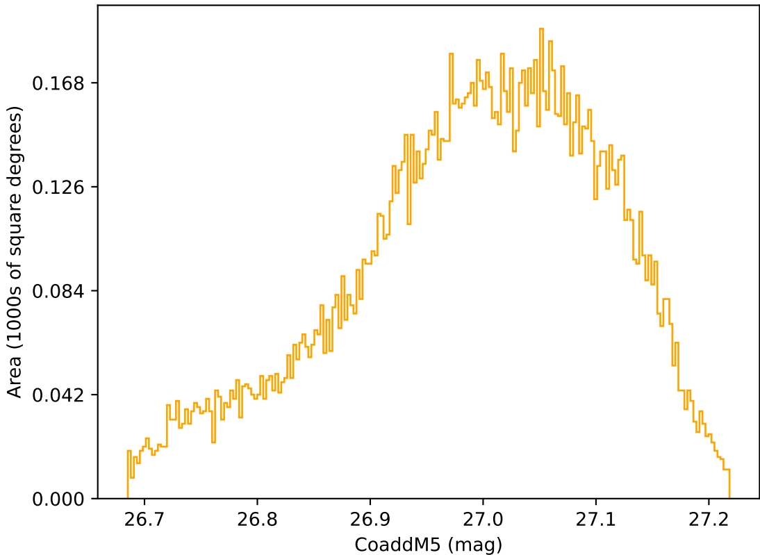
ddf_acor_sf15_ls40_lsr20_v3.4_10yrs WFD r band: CoaddM5
