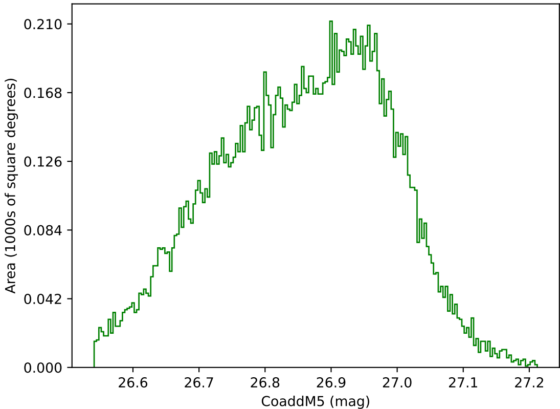
ddf_acor_sf15_lsf40_lsr20_v3.4_10yrs WFD g band: CoaddM5
