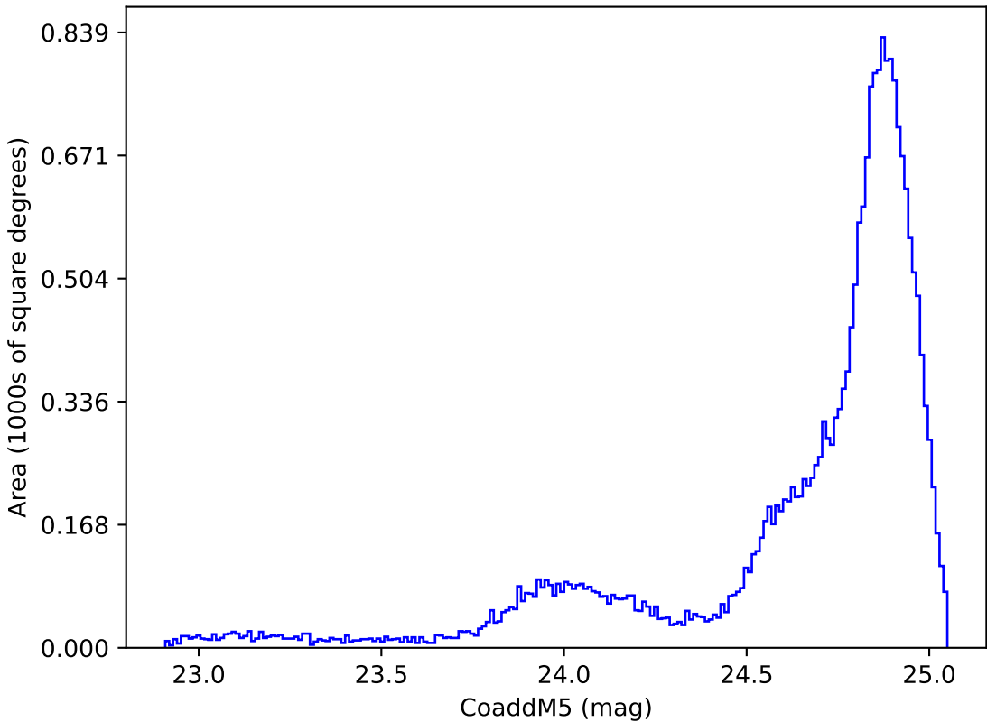
ddf_acor_sf15_lsf40_lsr20_v3.4_10yrs All sky y band: CoaddM5
