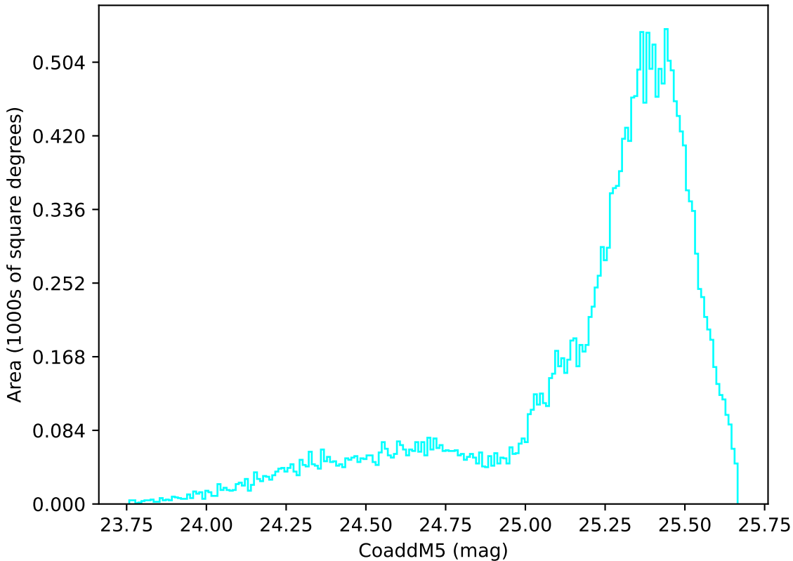
ddf_acor_sf15_lsf40_lsr20_v3.4_10yrs All sky u band: CoaddM5
