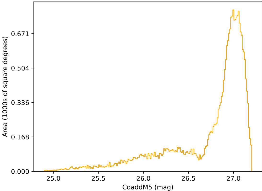
ddf_acor_sf15_lsf40_lsr20_v3.4_10yrs All sky r band: CoaddM5
