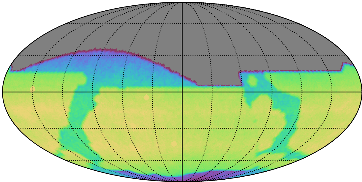
ddf_acor_sf15_lsf40_lsr20_v3.4_10yrs All sky i band: CoaddM5
