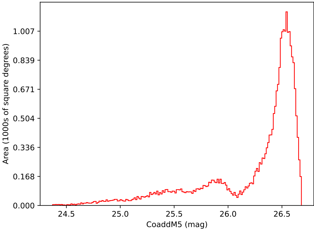
ddf_acor_sf15_lsf40_lsr20_v3.4_10yrs All sky i band: CoaddM5
