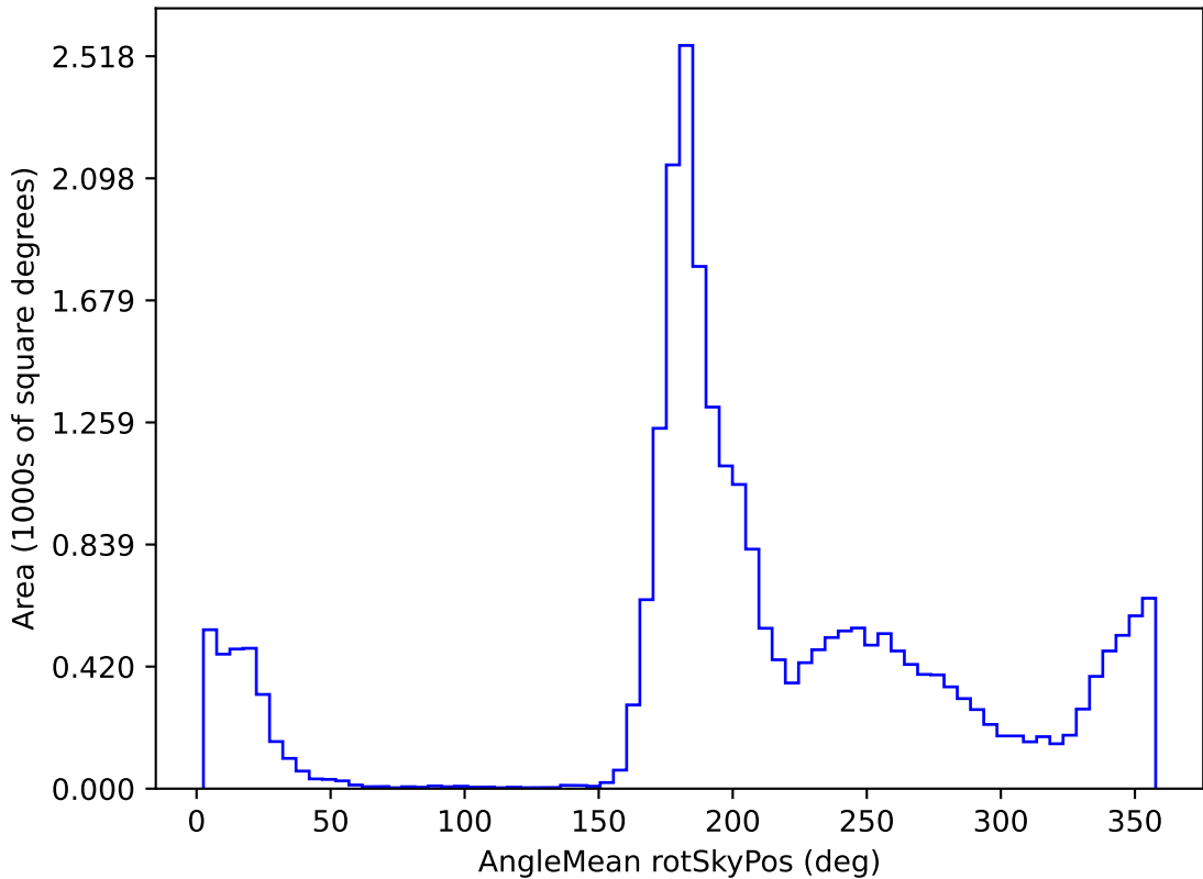
ddf_acor_sf15_lsf40_lsr20_v3.4_10yrs All sky i band: AngleMean rotSkyPos
