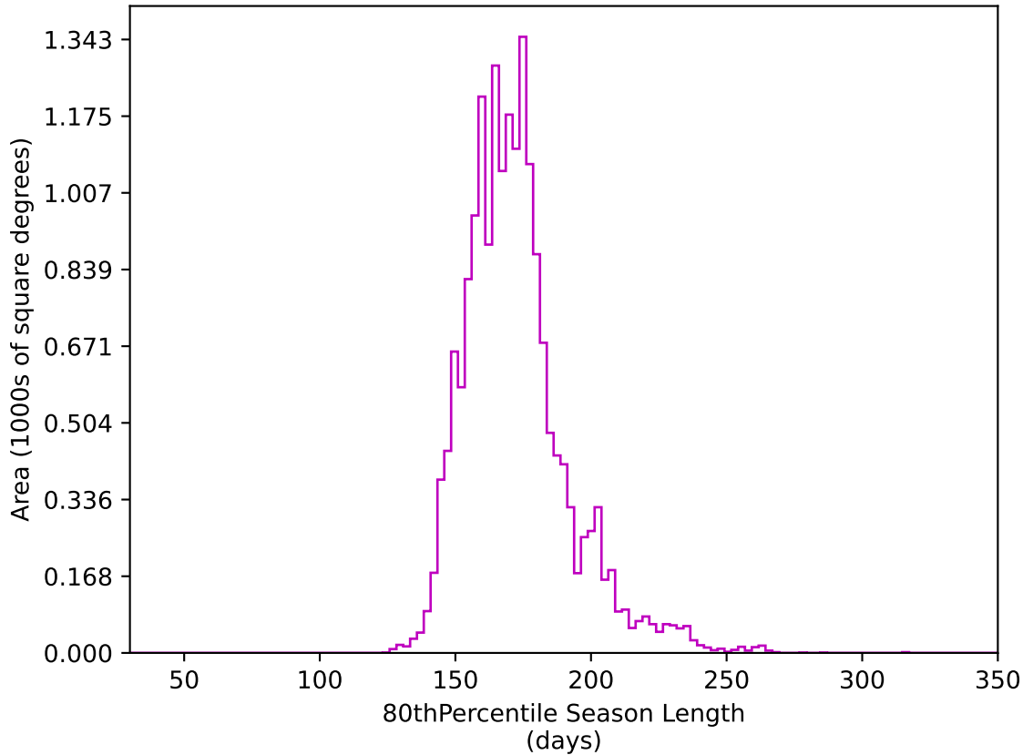
ddf_acor_sf15_lsf40_lsr20_v3.4_10yrs WFD z band: 80thPercentile Season Length
