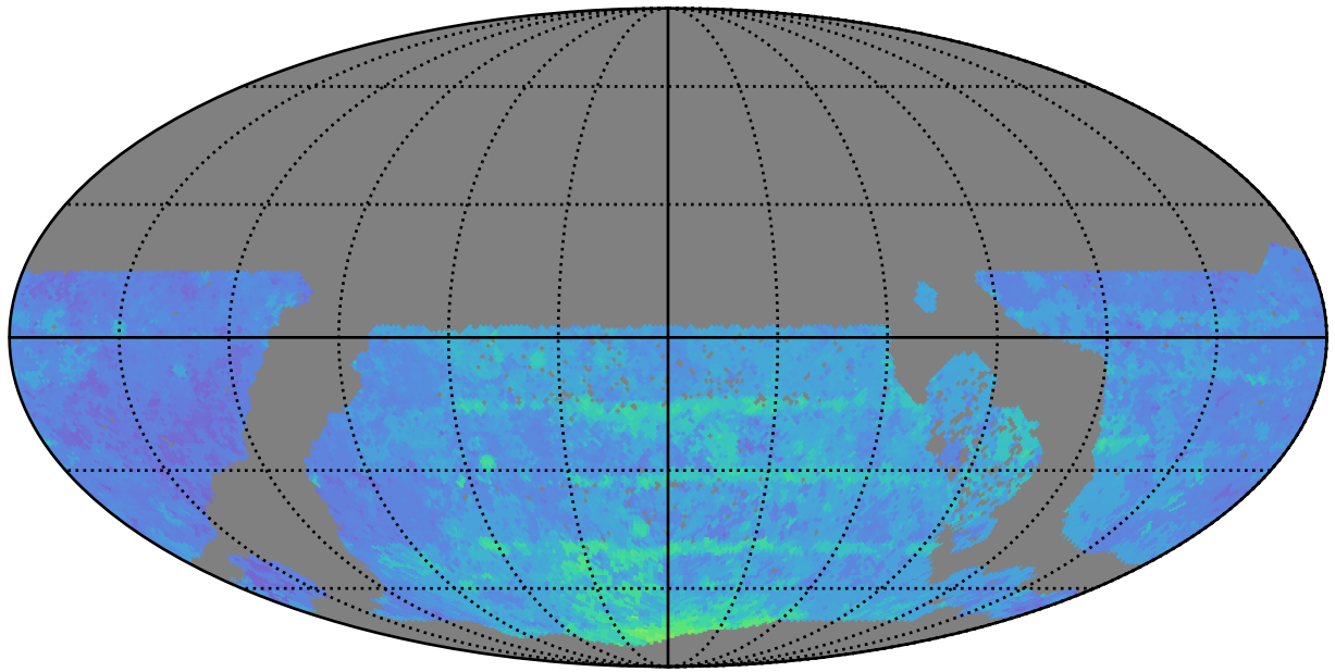
ddf_acor_sf15_lsf40_lsr20_v3.4_10yrs WFD y band: 80thPercentile Season Length
