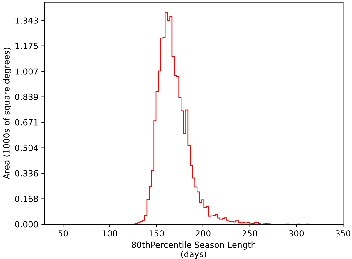
ddf_acor_sf15_lsf40_lsr20_v3.4_10yrs WFD i band: 80thPercentile Season Length
