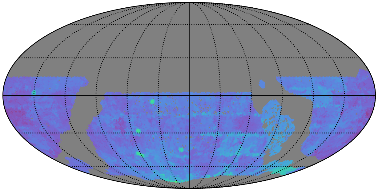
ddf_acor_sf15_lsf40_lsr20_v3.4_10yrs WFD g band: 80thPercentile Season Length
