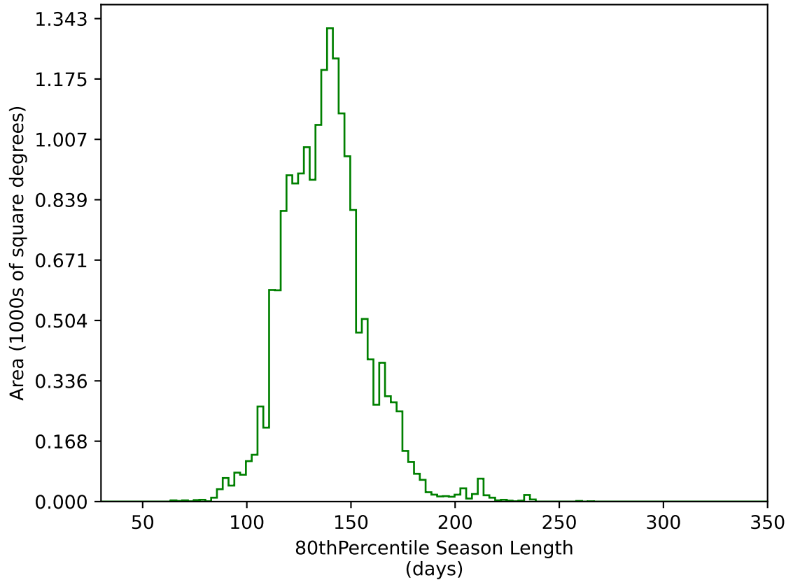
ddf_acor_sf15_lsf40_lsr20_v3.4_10yrs WFD g band: 80thPercentile Season Length
