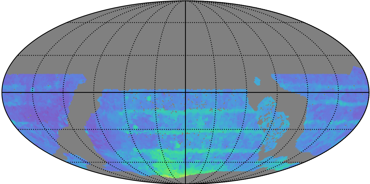
ddf_acor_sf15_lsf40_lsr20_v3.4_10yrs WFD all bands: 80thPercentile Season Length
