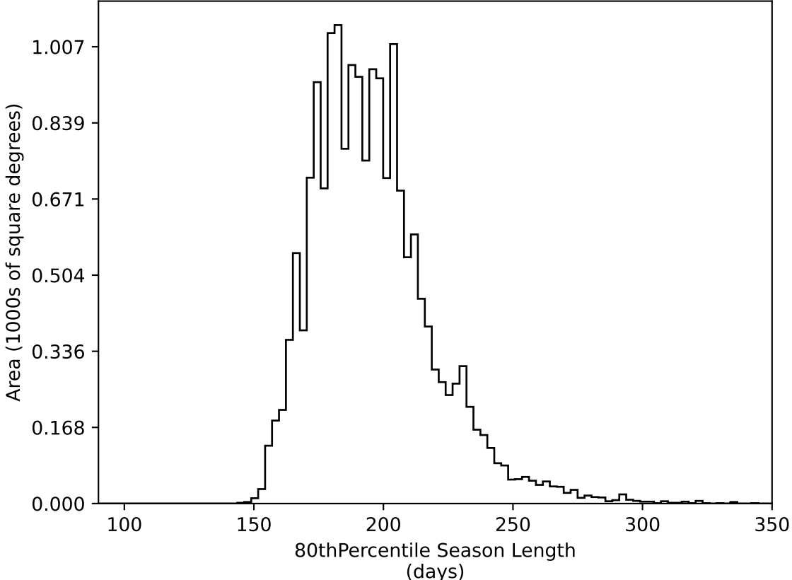
ddf_acor_sf15_lsf40_lsr20_v3.4_10yrs WFD all bands: 80thPercentile Season Length
