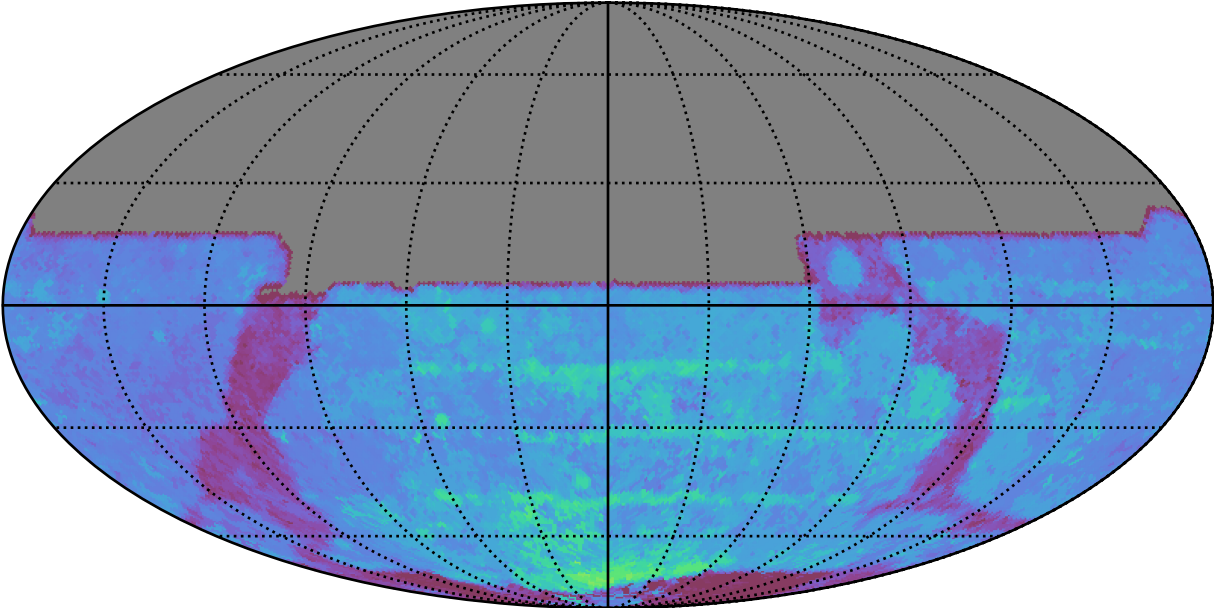
ddf_acor_sf15_lsf40_lsr20_v3.4_10yrs All sky y band: 80thPercentile Season Length
