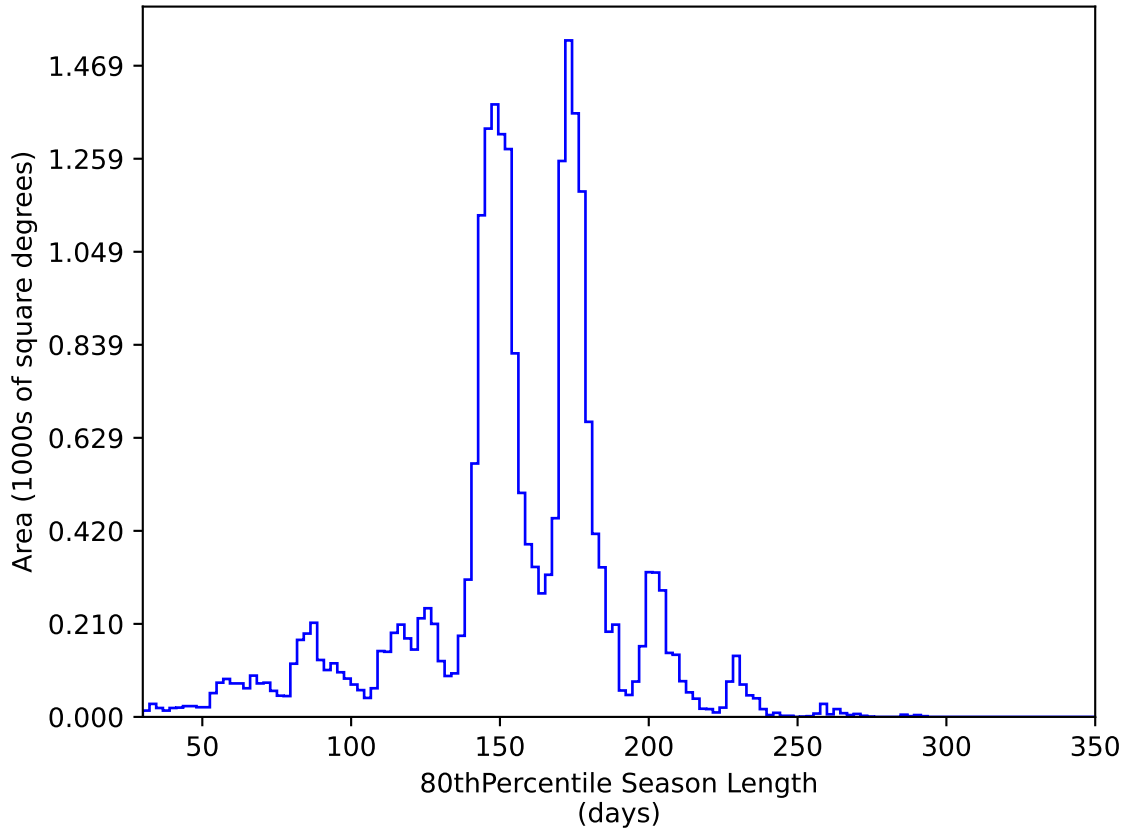
ddf_acor_sf15_lsf40_lsr20_v3.4_10yrs All sky y band: 80thPercentile Season Length
