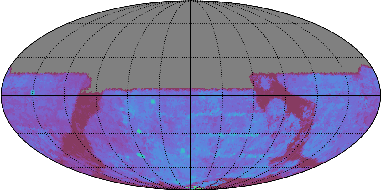
ddf_acor_sf15_lsf40_lsr20_v3.4_10yrs All sky u band: 80thPercentile Season Length
