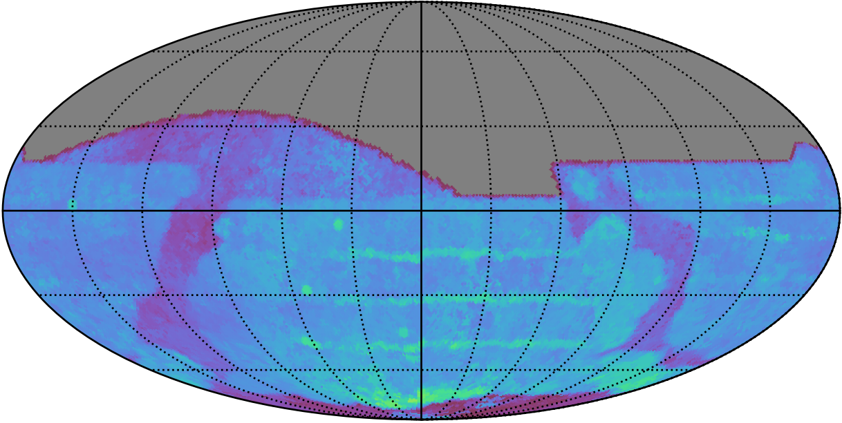
ddf_acor_sf15_lsf40_lsr20_v3.4_10yrs All sky r band: 80thPercentile Season Length
