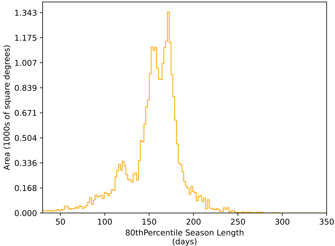
ddf_acor_sf15_lsf40_lsr20_v3.4_10yrs All sky r band: 80thPercentile Season Length
