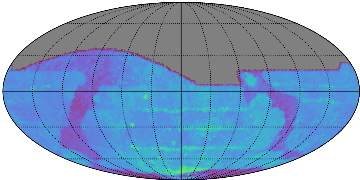
ddf_acor_sf15_lsf40_lsr20_v3.4_10yrs All sky i band: 80thPercentile Season Length
