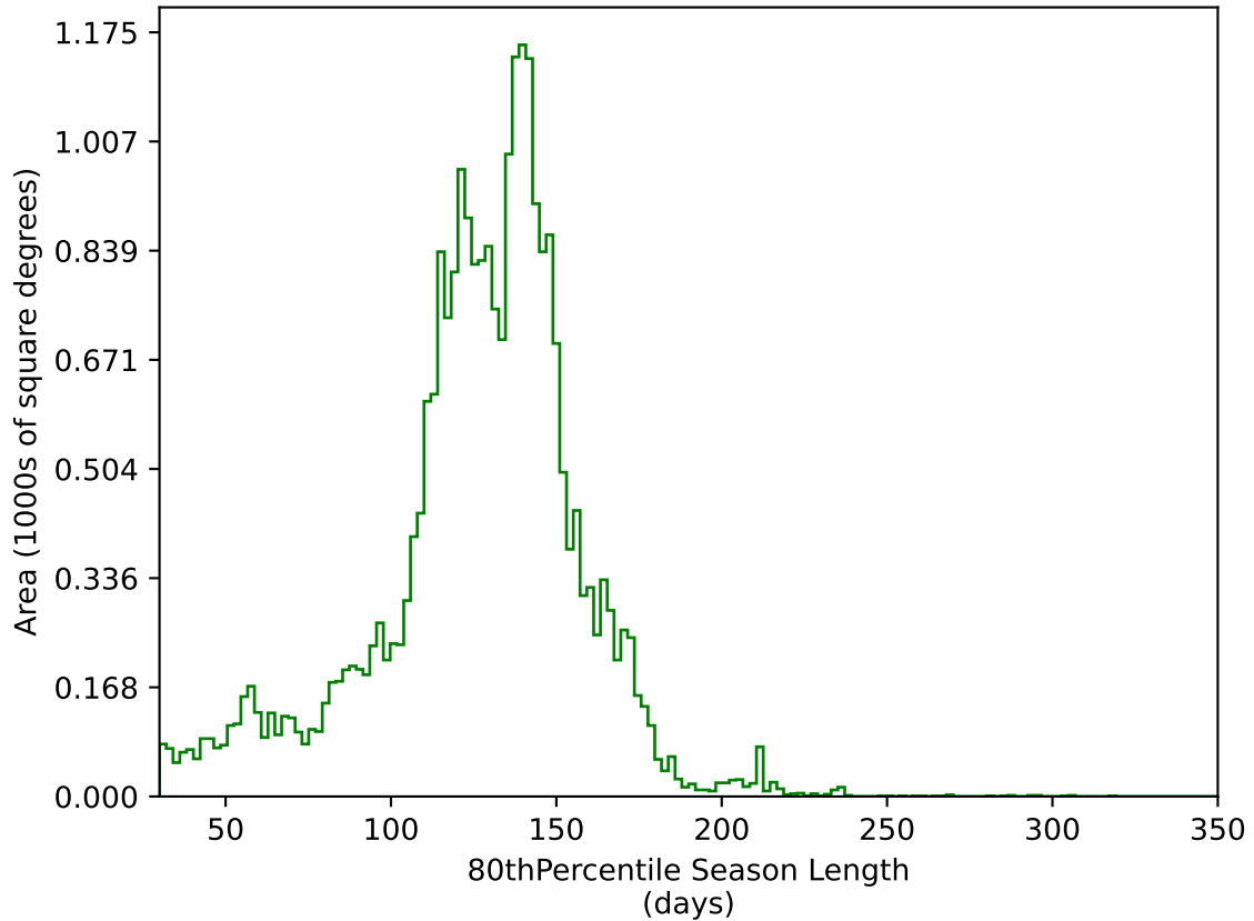
ddf_acor_sf15_lsf40_lsr20_v3.4_10yrs All sky g band: 80thPercentile Season Length
