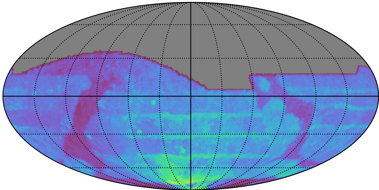
ddf_acor_sf15_lsf40_lsr20_v3.4_10yrs All sky all bands: 80thPercentile Season Length
