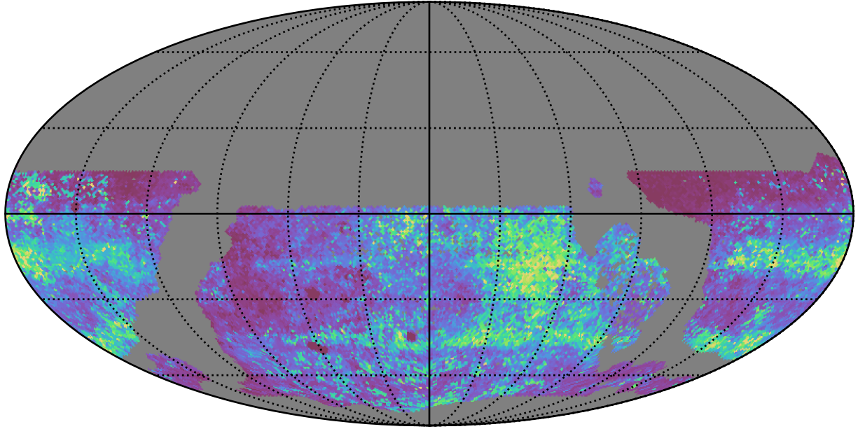
ddf_acor_sf15_lsf40_lsr20_v3.4_10yrs WFD zy bands: 75th Percentile Intranight Timespan
