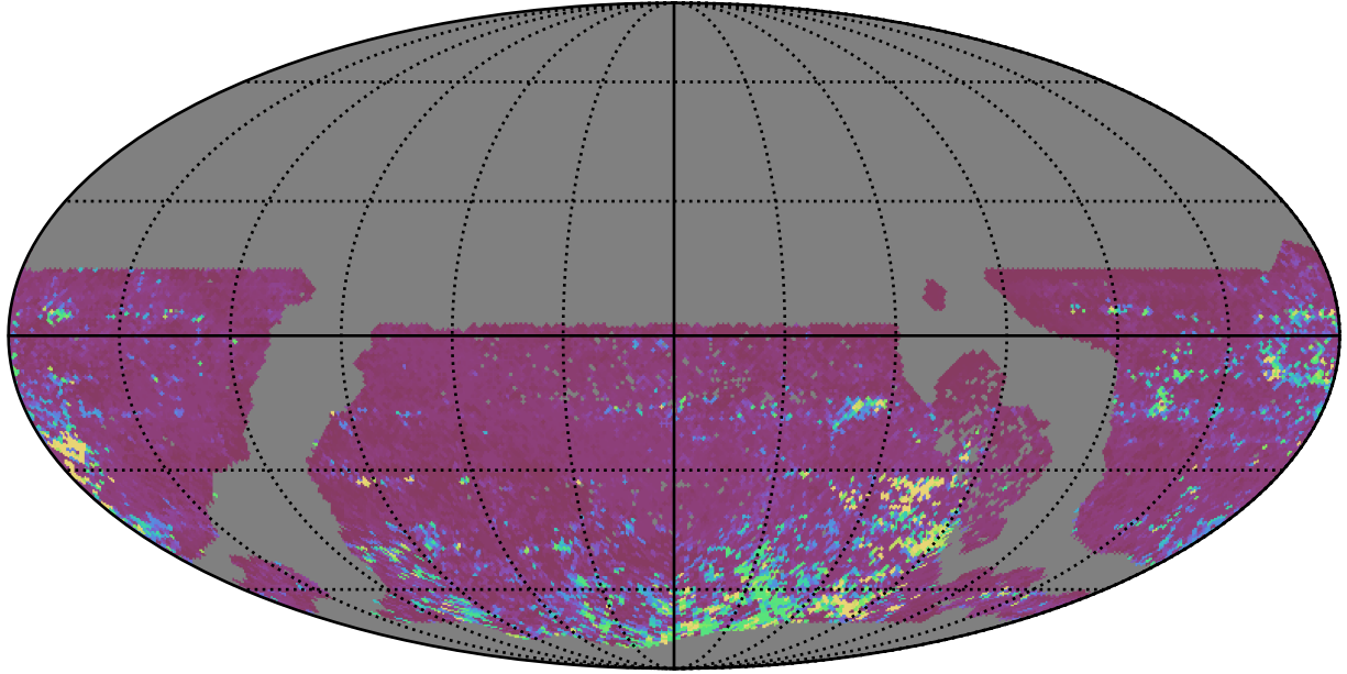
ddf_acor_sf15_lsf40_lsr20_v3.4_10yrs WFD z band: 75th Percentile Intranight Timespan
