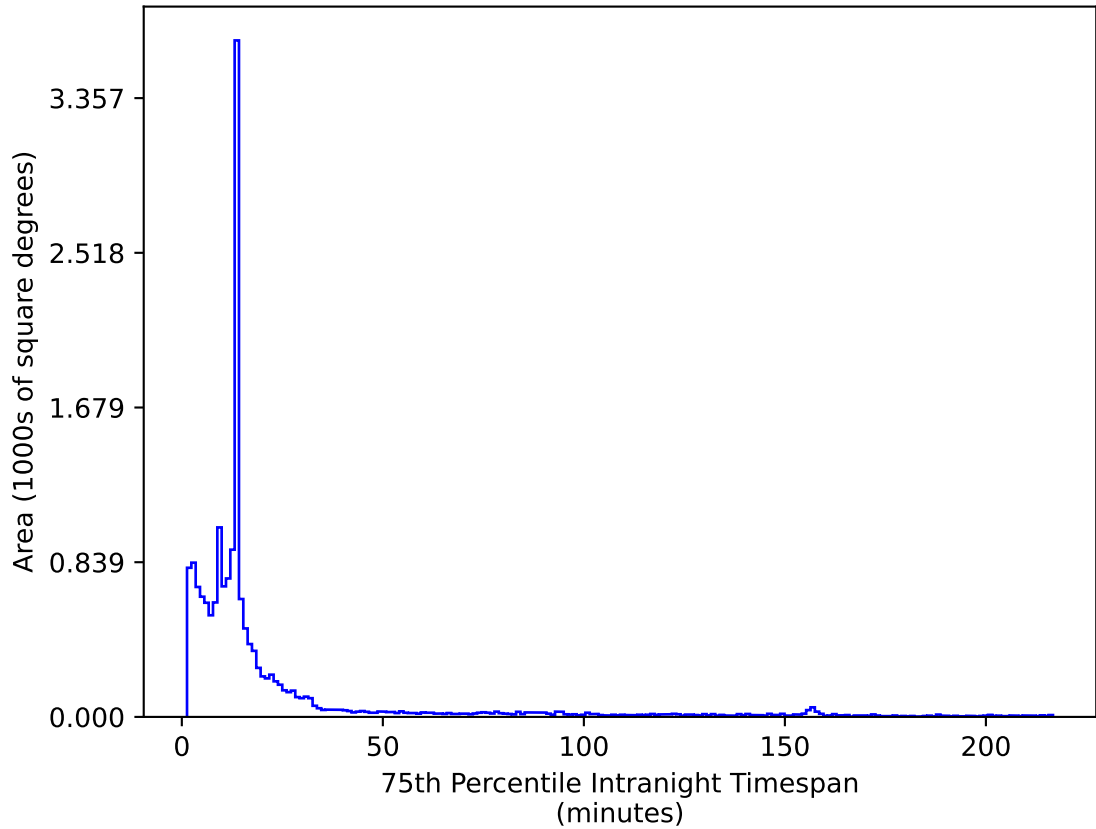
ddf_acor_sf15_lsf40_lsr20_v3.4_10yrs WFD z band: 75th Percentile Intranight Timespan
