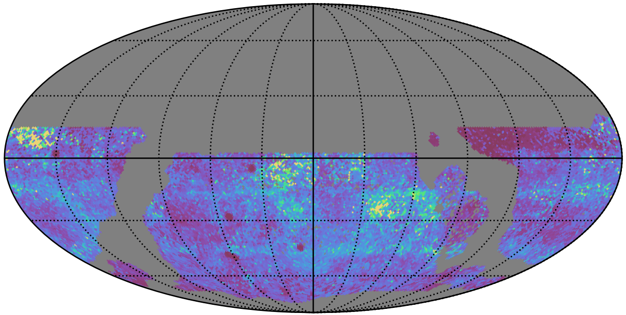
ddf_acor_sf15_lsf40_lsr20_v3.4_10yrs WFD y band: 75th Percentile Intranight Timespan
