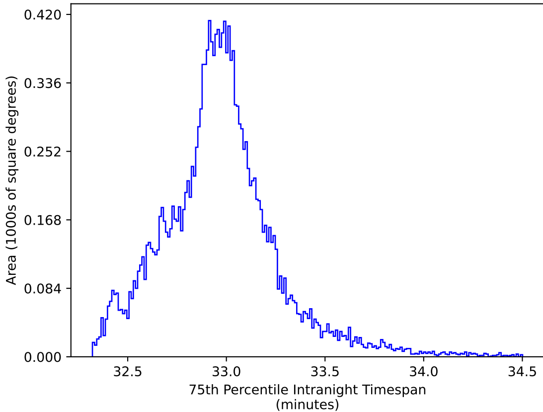
ddf_acor_sf15_lsf40_lsr20_v3.4_10yrs WFD y band: 75th Percentile Intranight Timespan
