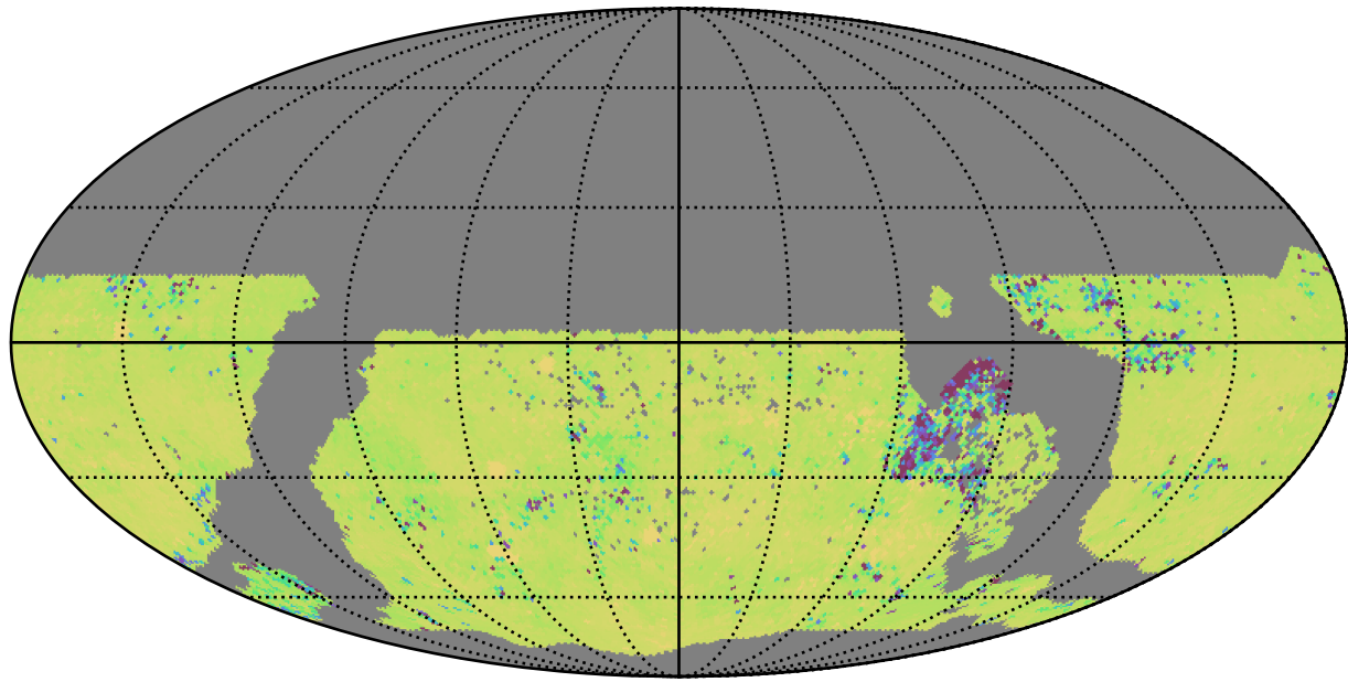
ddf_acor_sf15_lsf40_lsr20_v3.4_10yrs WFD ug bands: 75th Percentile Intranight Timespan
