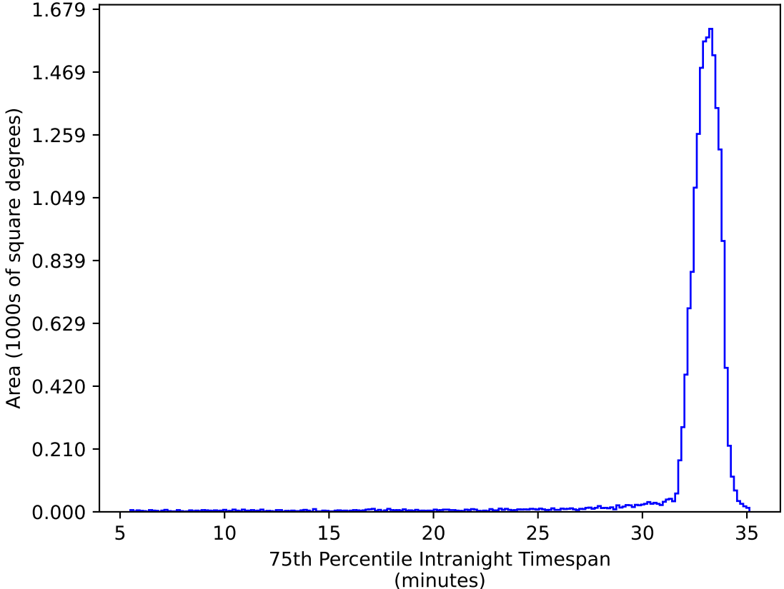
ddf_acor_sf15_lsf40_lsr20_v3.4_10yrs WFD ug bands: 75th Percentile Intranight Timespan
