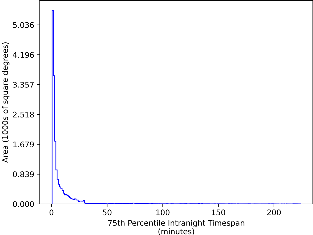
ddf_acor_sf15_lsf40_lsr20_v3.4_10yrs WFD u band: 75th Percentile Intranight Timespan
