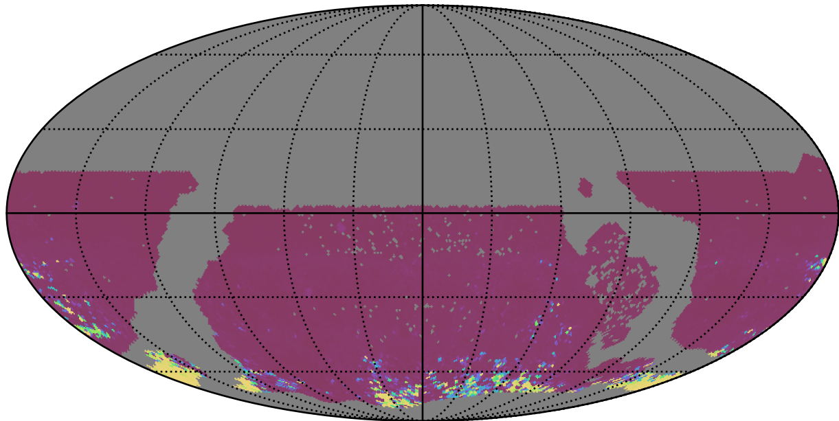
ddf_acor_sf15_lsf40_lsr20_v3.4_10yrs WFD ri bands: 75th Percentile Intranight Timespan
