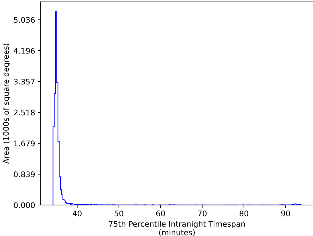
ddf_acor_sf15_lsf40_lsr20_v3.4_10yrs WFD ri bands: 75th Percentile Intranight Timespan
