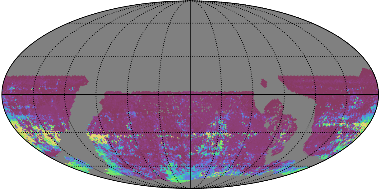
ddf_acor_sf15_lsf40_lsr20_v3.4_10yrs WFD r band: 75th Percentile Intranight Timespan
