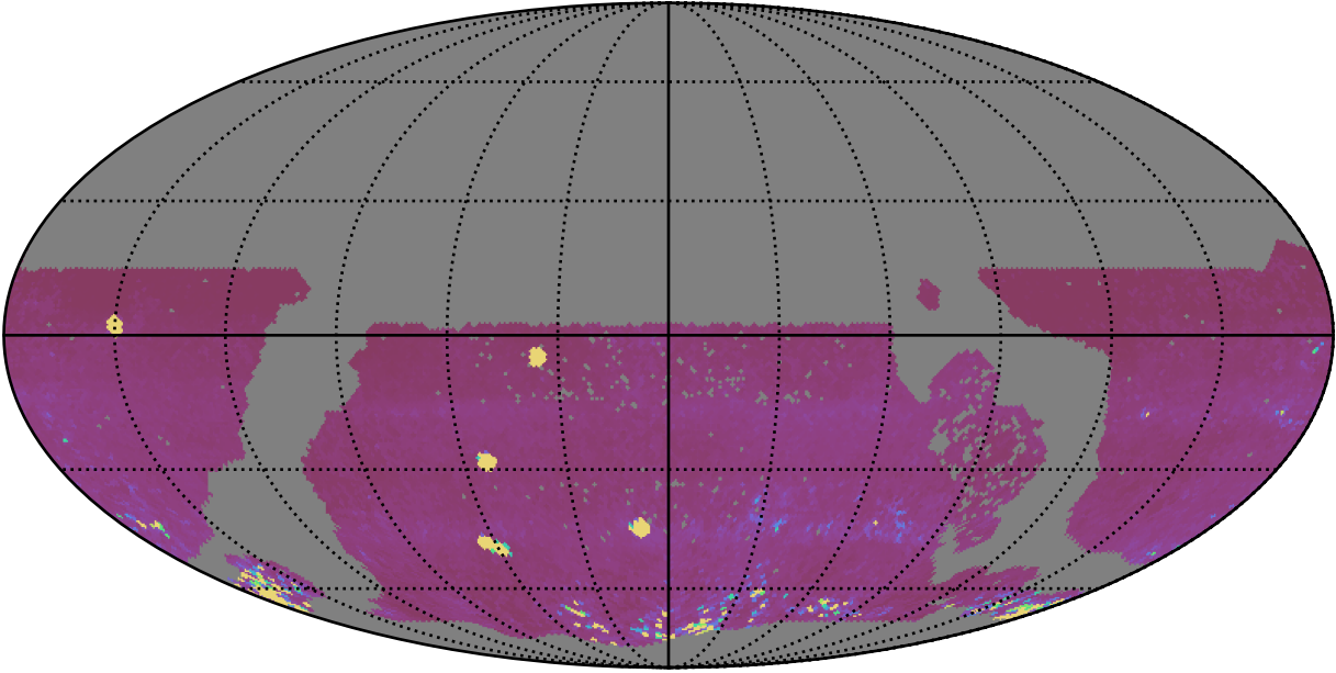
ddf_acor_sf15_lsf40_lsr20_v3.4_10yrs WFD iz bands: 75th Percentile Intranight Timespan
