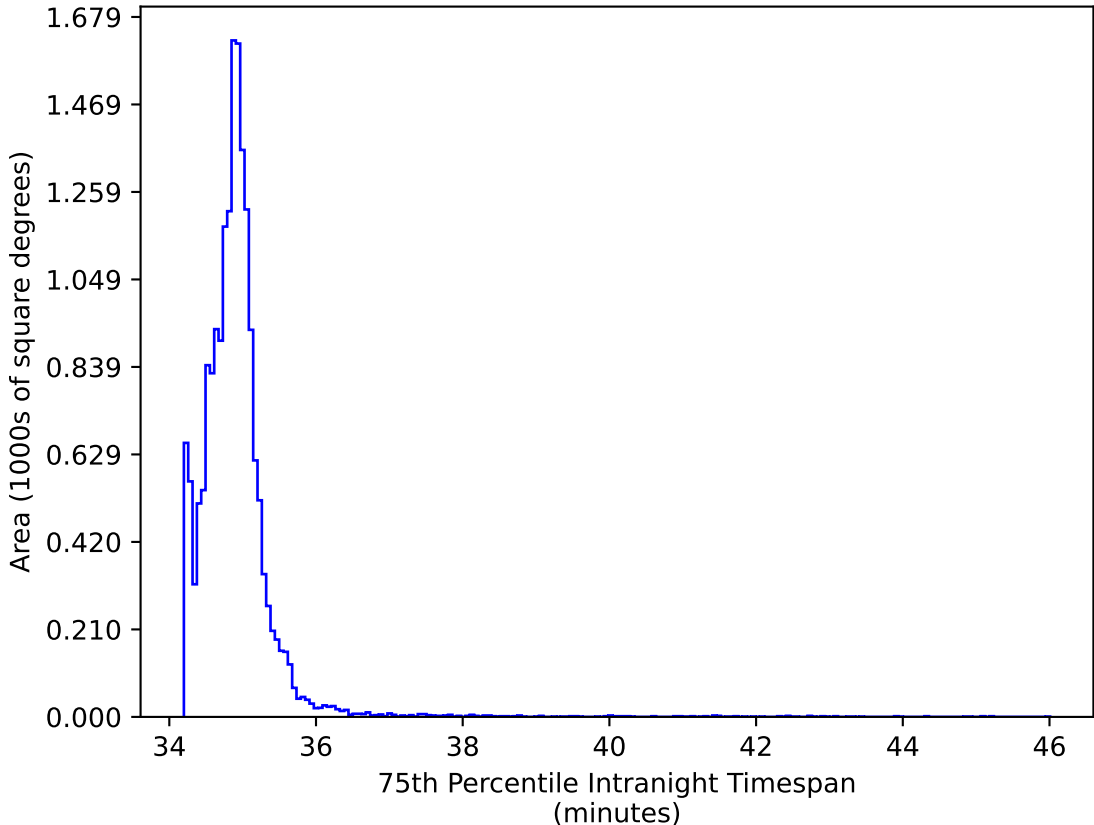
ddf_acor_sf15_lsf40_lsr20_v3.4_10yrs WFD iz bands: 75th Percentile Intranight Timespan
