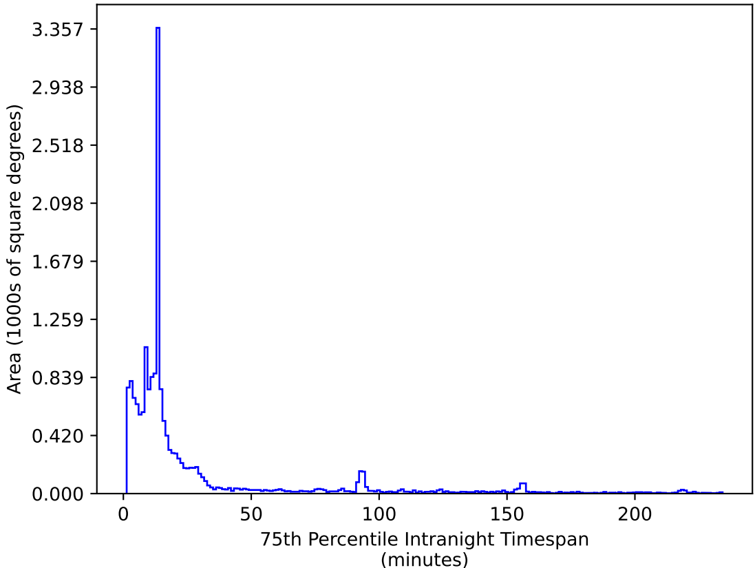
ddf_acor_sf15_lsf40_lsr20_v3.4_10yrs WFD i band: 75th Percentile Intranight Timespan
