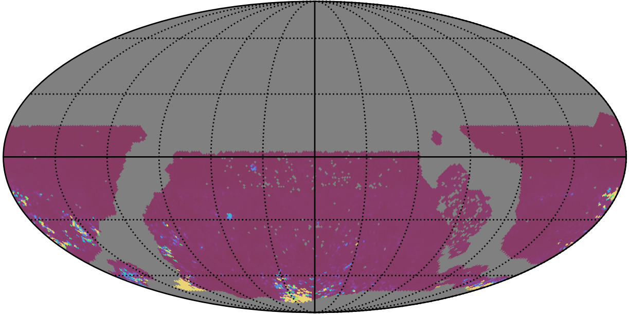
ddf_acor_sf15_lsf40_lsr20_v3.4_10yrs WFD gr bands: 75th Percentile Intranight Timespan
