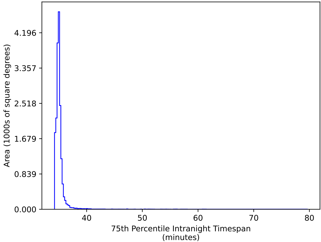
ddf_acor_sf15_lsf40_lsr20_v3.4_10yrs WFD gr bands: 75th Percentile Intranight Timespan
