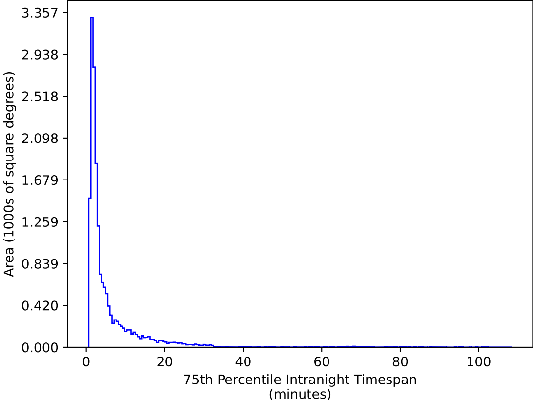
ddf_acor_sf15_lsf40_lsr20_v3.4_10yrs WFD g band: 75th Percentile Intranight Timespan
